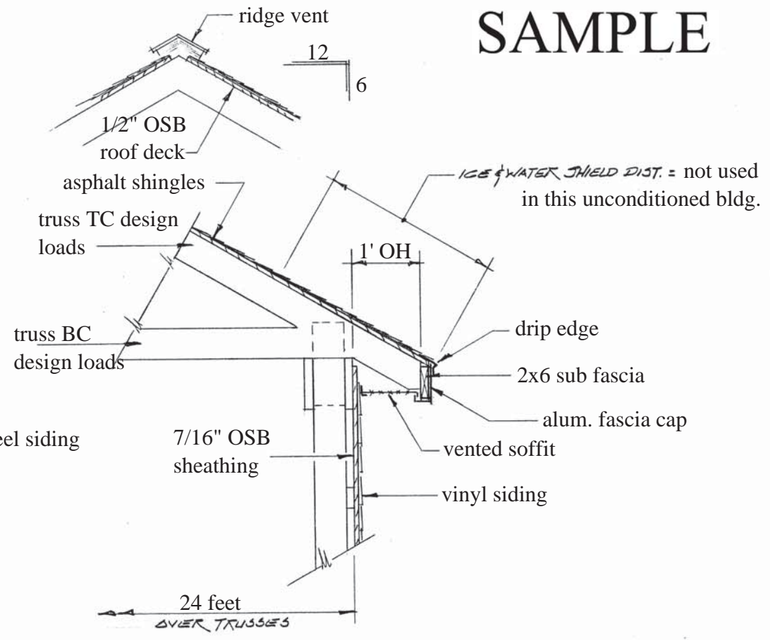
UNHEATED POST FRAME WALL DETAIL w/ SHINGLE ROOF & SIDING SCALE: NONE
