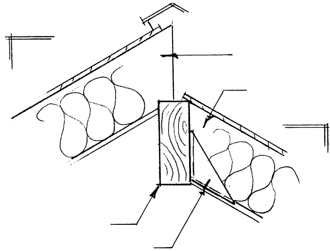
RAFTERS W/ RIDGE BEAM & CATHEDRAL CEILING
