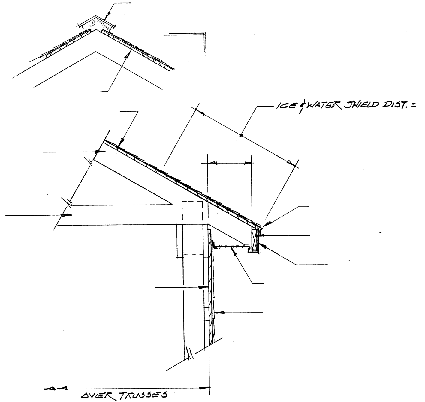
UNHEATED POST FRAME WALL DETAIL W/ SHINGLE ROOF & SIDING SCALE: NONE
